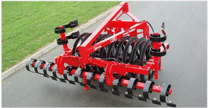
1.50 m with 4.00 m Spring-Board in transport position.
