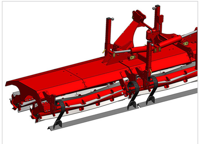
Cutter-Board - spring mounted levelling bar.
