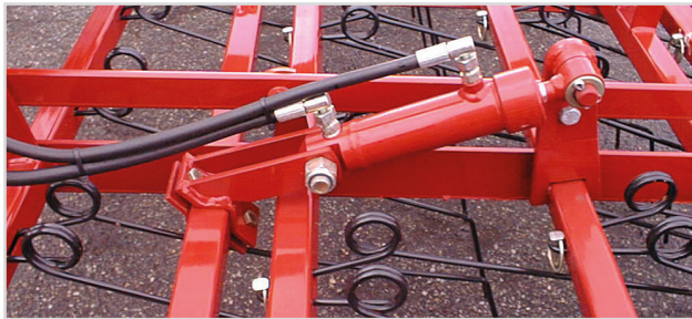
Hydraulically adjustable tine pressure
