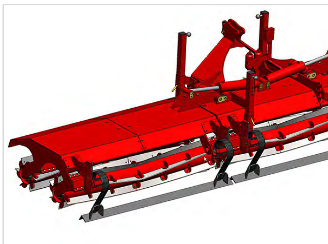
Cutter-Board - spring mounted levelling bar.
