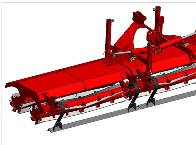
Cutter-Board - spring mounted levelling bar.
